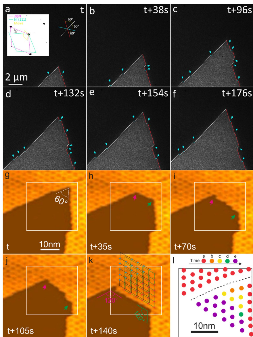
Figure 12. Shape of concave corners between merging domains growing under the influence of a strong film–substrate interaction. (a–f) Sequence of in situ PEEM images recorded during h BN growth on Ni(111) at 640 °C under a total pressure of 4.7 \times 10^{-6} Pa ( \text{BH}_3\text{NH}_3 ) showing MMK creation on zigzag edges of h BN. The inset in (a) shows a low-energy electron diffraction (LEED) (50 eV) pattern recorded from the observed region. Rhombuses with different colors: purple, h BN; green, Ni(111); yellow, moiré superstructure. The different direction of zigzag edges is highlighted by a different color. Note that the angles at MMK sites, which are highlighted in (a)–(f) by blue arrows, measure 120^\circ and remain unchanged during growing. The growth behavior of h BN on Ni is similar to the one of graphene on Rh (refer to Figure 9). (g–k) In situ STM images recorded during h BN growth on Rh(111) at 700 °C at a pressure of 1.2 \times 10^{-7} Pa using borazine as precursor. 81 The STM images were recorded at a sample voltage of V_b = 1.0 V and a tunneling current of I_t = 0.05 nA. The green and black grids in (k) indicate the lattice of the moiré pattern formed between h BN and the Rh(111). Note that red and blue dots in (k) highlight depression areas (strong adsorption region) in the moiré supercell. The purple arrows highlight the concave corner at which a GB is formed. The green arrows highlight a concave corner where coalescence is seamless. (l) Schematic representation of the time-dependent changes of the domain shown in (g)–(k). The superimposed colored dots correspond to depression areas in the moiré supercell and were extracted from the area indicated by a white square in frames (g)–(k). The dashed line in (l) indicates the position of the GB. Note that the growth behavior of h BN is similar to graphene on Rh (the kink creation at the edge occurs in units of the moiré lattice) and the angle of the concave corners remains the same during coalescence.
