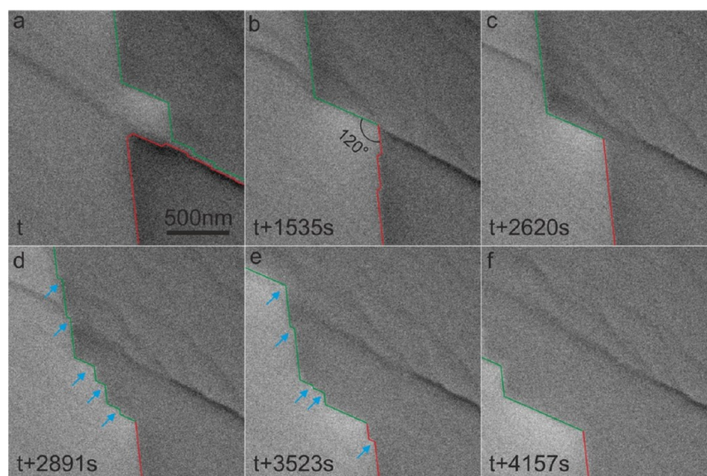
Figure 9. Time-lapse image series recorded during the coalescence of well-aligned domains on Rh(111) at 900 °C and a total pressure of 25 Pa ( C_2H_4/H_2 = 1:100 ). The green and red lines highlight the growth fronts of the coalescing domains. The intersection corners remain at an angle of 120° throughout the coalescence process. Note that the angles of MMK sites, which are highlighted in (d) and (e) by blue arrows, are also 120°.
