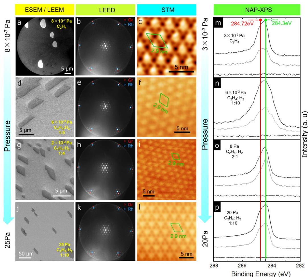
Figure 1. Graphene growth on Rh(111) under different pressure. (a, d, g, j) In situ LEEM/ESEM images obtained during growth of graphene domains by CVD from C_2H_4 on Rh(111) at constant temperature ( T = 900\text{ }^\circ\text{C} ). Growth condition (pressure, C_2H_4/H_2 ): (a) 8 \times 10^{-7} Pa, pure C_2H_4 ; (d) 6 \times 10^{-3} Pa, 1:5; (g) 2 \times 10^{-2} Pa, 1:4 and (j) 25 Pa, 1:10. The corresponding LEED patterns and STM images of graphene grown within the ESEM/LEEM chamber at different condition are shown in (b, c), (e, f), (h, i), and (k, l), respectively. In (b), (e), (h), and (k), the six inner diffraction spots (marked by blue circles) are from Rh(111), and the outer spots (marked by red circles) are from graphene. The green rhombuses in (c), (f), (i), and (l) indicate the (12 \times 12)_C on (11 \times 11)_{Rh} moiré superstructure. (m)–(p) show C_{1s} spectra recorded during graphene growth on Rh(111) at 900\text{ }^\circ\text{C} under different gas environments. (m) Exposure to pure C_2H_4 at 3 \times 10^{-3} Pa; (n) exposure to a 1:10 C_2H_4/H_2 gas mixture at 6 \times 10^{-2} Pa; (o) exposure to a 2:1 C_2H_4/H_2 gas mixture at 8 Pa; (p) exposure to a 1:10 C_2H_4/H_2 gas mixture at 20 Pa; binding energies of the main components were derived by spectral deconvolution and are indicated in the figure.
