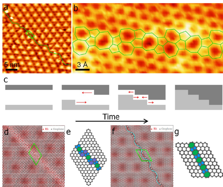
Figure 10. Postgrowth STM imaging reveals the GB structure on Rh(111). (a) STM overview image (28 nm × 28 nm) of the graphene GB (highlighted by a green line) observed on Rh(111) after CVD growth inside the ESEM chamber at a total pressure of 25 Pa ( C_2H_4/H_2 = 1:100 ). (b) Atomically resolved graphene GB (magnification of the green square in (a)) together with a superimposed GB model. The GB model is realized through a linear chain of abutting pentagon pairs–octagon–pentagon pairs–heptagon pairs. (c) Schematic representation of the formation of a stair-stepped GB. Red arrows indicate the direction of kink growth. (d and f) Schematic representations of the relationship between the moiré pattern of aligned domains and the resulting GB with two different stitching edges. The corresponding atomistic models of GB structures are depicted in (e) and (g). A sinusoidal curve (blue) is added in (g) as a guide to the eye, to facilitate the comparison of the moiré period on both sides of the GB. Tunneling conditions: (a) V_s = 1 V, I_t = 0.3 nA; (b) V_s = 0.5 V, I_t = 0.5 nA.
