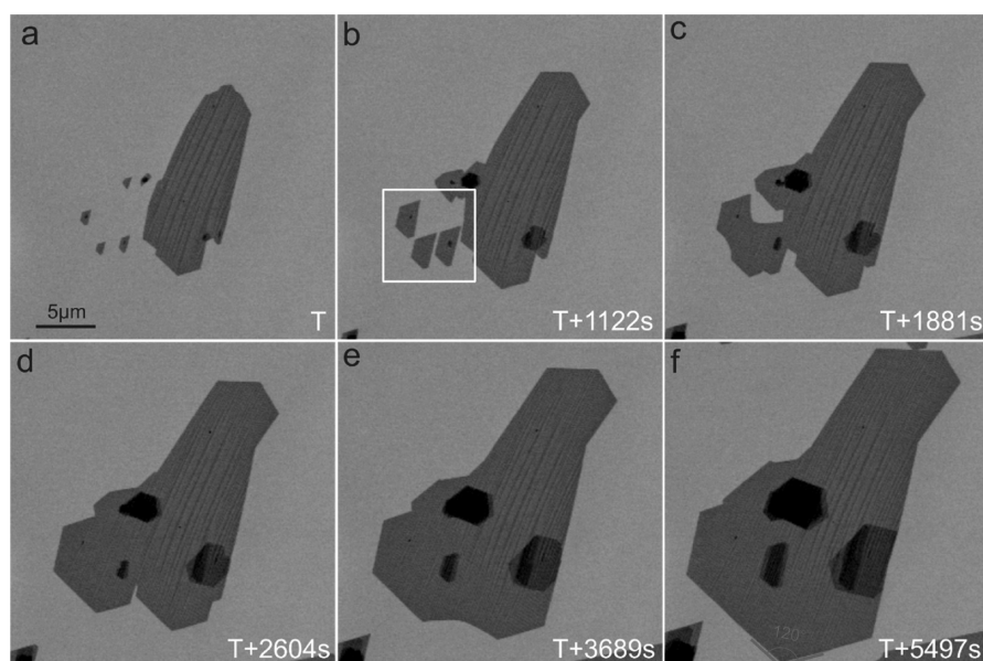
Figure 4. In situ ESEM images recorded at 900 °C showing the nucleation and coalescence of graphene on Pt(111) at different growing times. The growing graphene sheets are characterized by a dark contrast. The domains enclosed by a white rectangle in (b) show a slight misalignment (a magnified image showing the misalignment is presented in Figure SI 4).
