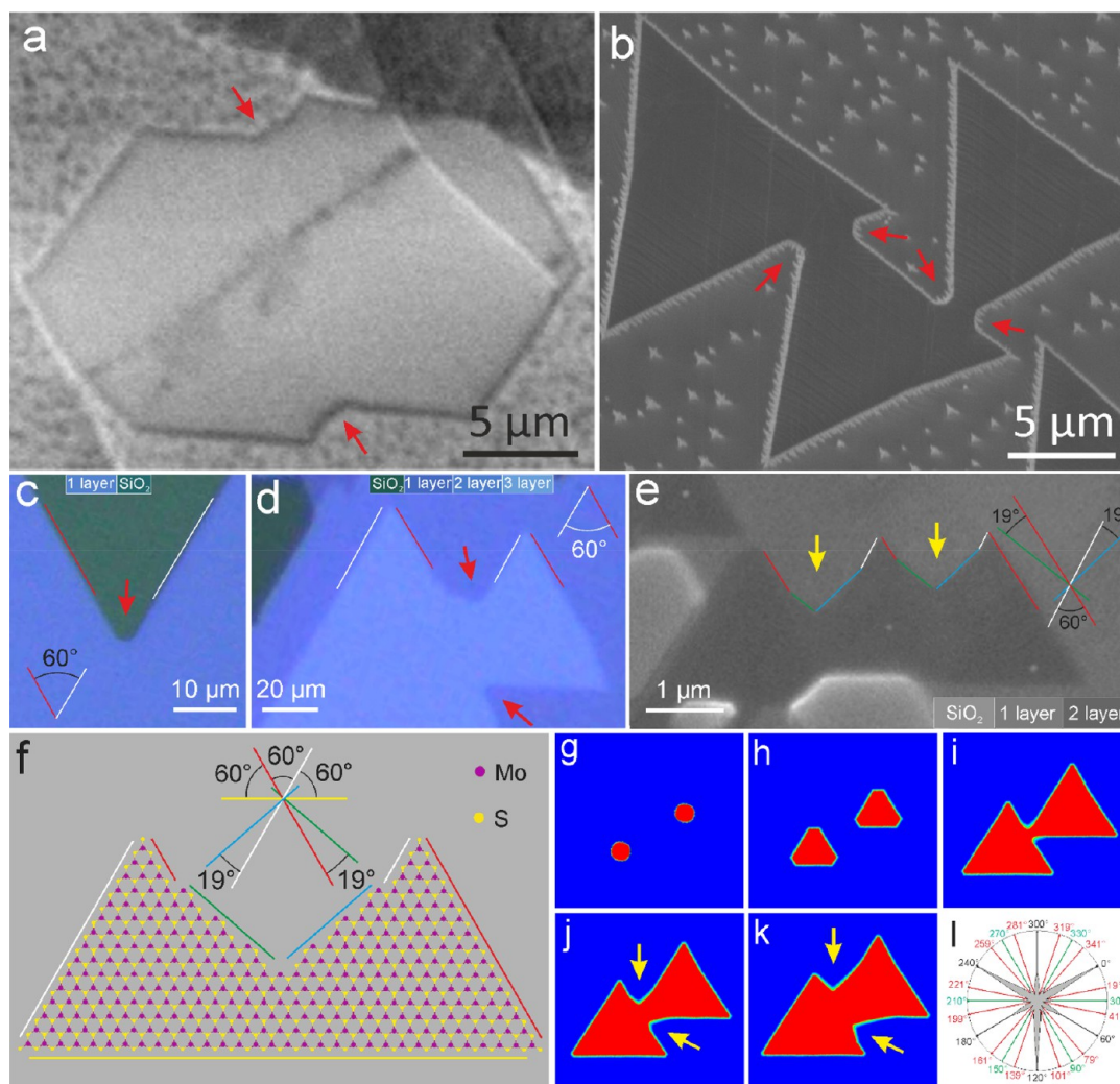
Figure 11. Shape of concave corners between coalescing domains in weak film–substrate interaction systems. (a) Scanning electron microscopy (SEM) image showing the coalescence of aligned domains graphene on Cu. (b) SEM image showing coalescence of aligned hBN on Cu. (c, d) Optical image of concave corner between aligned MoS 2 domains grown on SiO 2 . The red arrows indicate rounded concave corners. (e) SEM image showing the appearance of 19.1° edges at concave corners of aligned MoS 2 domains. (f) Schematic view showing the 19.1° edge and morphology evolution during coalescence. (g–k) Phase-field-theory simulation of the coalescence of aligned MoS 2 domains and corresponding polar plots (l) showing the logarithm of relaxation time along different growth directions. A smaller relaxation time represents a lower growth barrier and thus a higher growth rate of an edge. Red color represents MoS 2 ; blue color represents the uncovered substrate. The yellow arrows indicate appearance of 19.1° edges at concave corners. In (c), (d), and (e), the number of layers can be abstracted by comparing the contrast in the images with the contrast legend in the respective panels.
