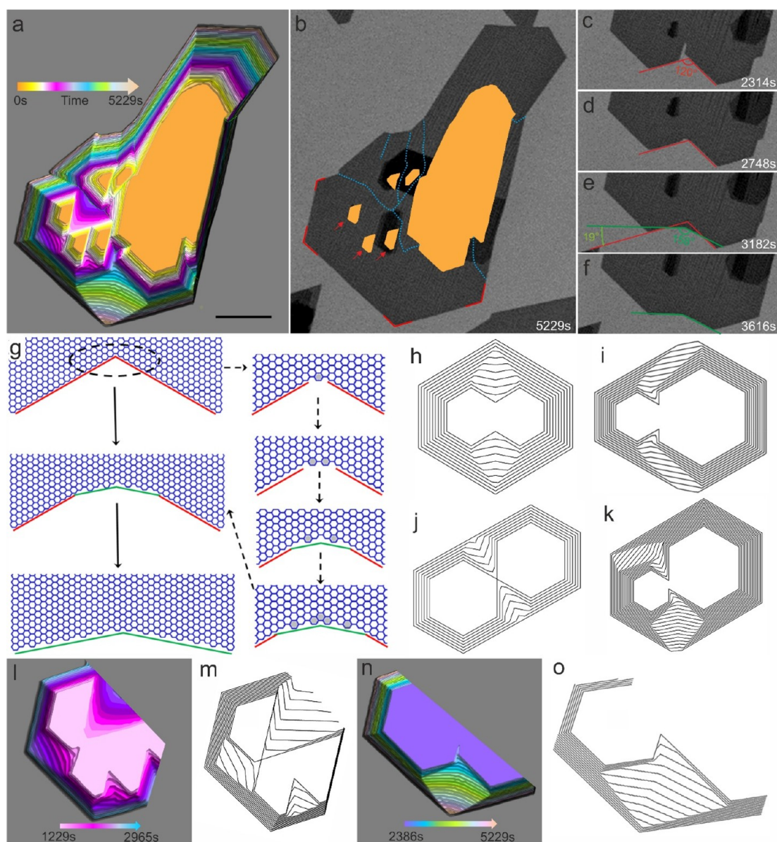
Figure 5. ESEM imaging of graphene growth on Pt(111) at 900 °C and KWC simulation of the shape evolution during the coalescence process. (a) Shape evolution of the graphene domains during coalescence, reproduced as color-coded superposition of outlines that were abstracted from images recorded during a 5300 s interval (Supporting Movie 3). The scale bar measures 5 \mu\text{m} . (b) Representation of the graphene GBs after coalescence. The blue dashed lines in (a) and (b) indicate the motion trajectory of the intersection point of misaligned graphene domains, which are responsible for GB formation during coalescence. The orange color-coded domains in (b) highlight the shape of graphene at the beginning of the recording. (c–f) Sequence of images showing the appearance of new edges at the concave corner during coalescence (the initial angle of the concave corner is highlighted by red lines, whereas the new edge angle is depicted in green). (g) Atomistic model of the growth process of a concave corner with an angle of 120° and zigzag edges in the case of well-aligned graphene domains. (h–k) KWC simulation of the shape evolution of well-aligned domains that coalesce from different directions and present a concave corner with an angle of either 120° (h) or 60° (i–k). (l) Superposition capturing the area of coalescence from three aligned domains marked by red arrows in (b). The outlines of growing domains are color-coded according to the growth time provided in the color legend. (n) Shape evolution of the graphene, reproduced as color-coded superposition of outlines that were abstracted from a sequence of in situ ESEM images (c–f). The corresponding coalescing processes shown in (l) and (n) are simulated by our modified KWC and presented in (m) and (o).
